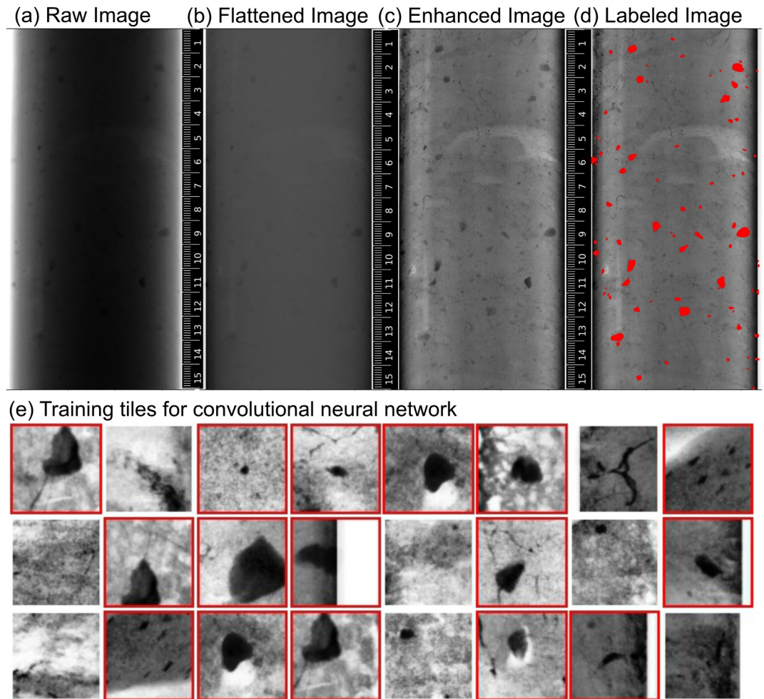
Figure 2. Image processing steps and training set creation. (a) Example of a 16-bit, 15-cm raw X-ray image from the pass-through X-Ray Imager. (b) A “flatten” function is applied to the raw X-ray image so that the geometry of the core does not interfere with the brightness contrast of the image. (c) The flattened X-ray image is then enhanced using the Scikit-image Contrast Limited Adaptive Histogram Equalization. (d) Red polygons are then drawn over the IRD grains, which labels them in the image. (e) The labeled image is then broken up into a series of 128 \times 128 -pixel square training “tiles.” Tiles with a red border are training images with an IRD grain at the center pixel. Tiles without a red border are training images that do not have IRD grains at the center pixel. Note, some of these “non-IRD” training images have targeted features such as pyritized burrows (in the top right). IRD, iceberg rafted debris.
